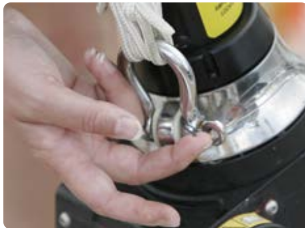
Check shackles are seized with wire or a zip tie
